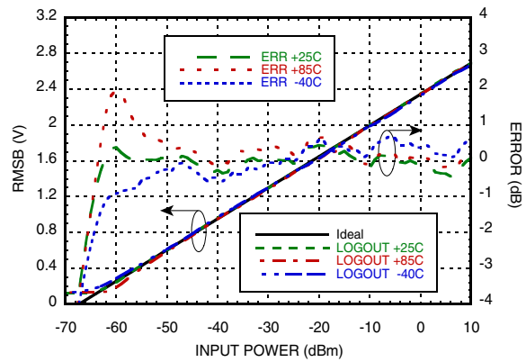
RMSB & Error vs. Pin @ 100 MHz [1]
