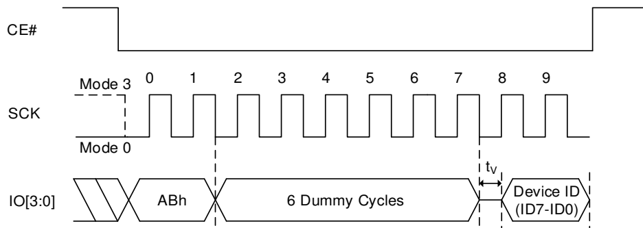
Figure 8.43 Read Product Identification Sequence In QPI Mode
