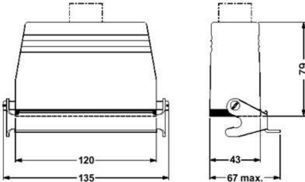
Dimensioned drawing
