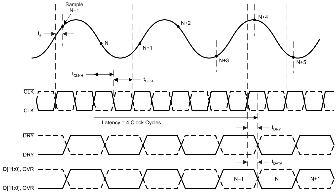
Figure 3. Timing Diagram
