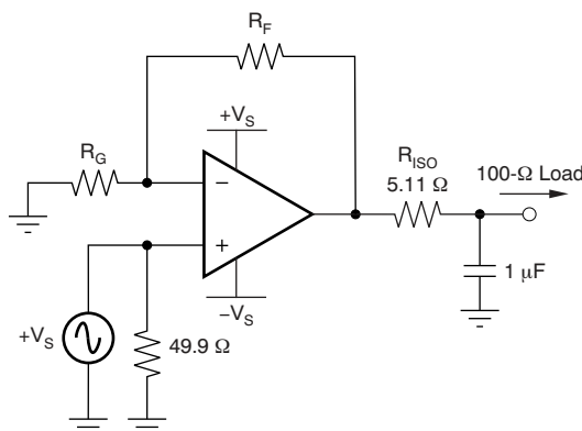
Figure 42. Resistor To Isolate Capacitive Load
