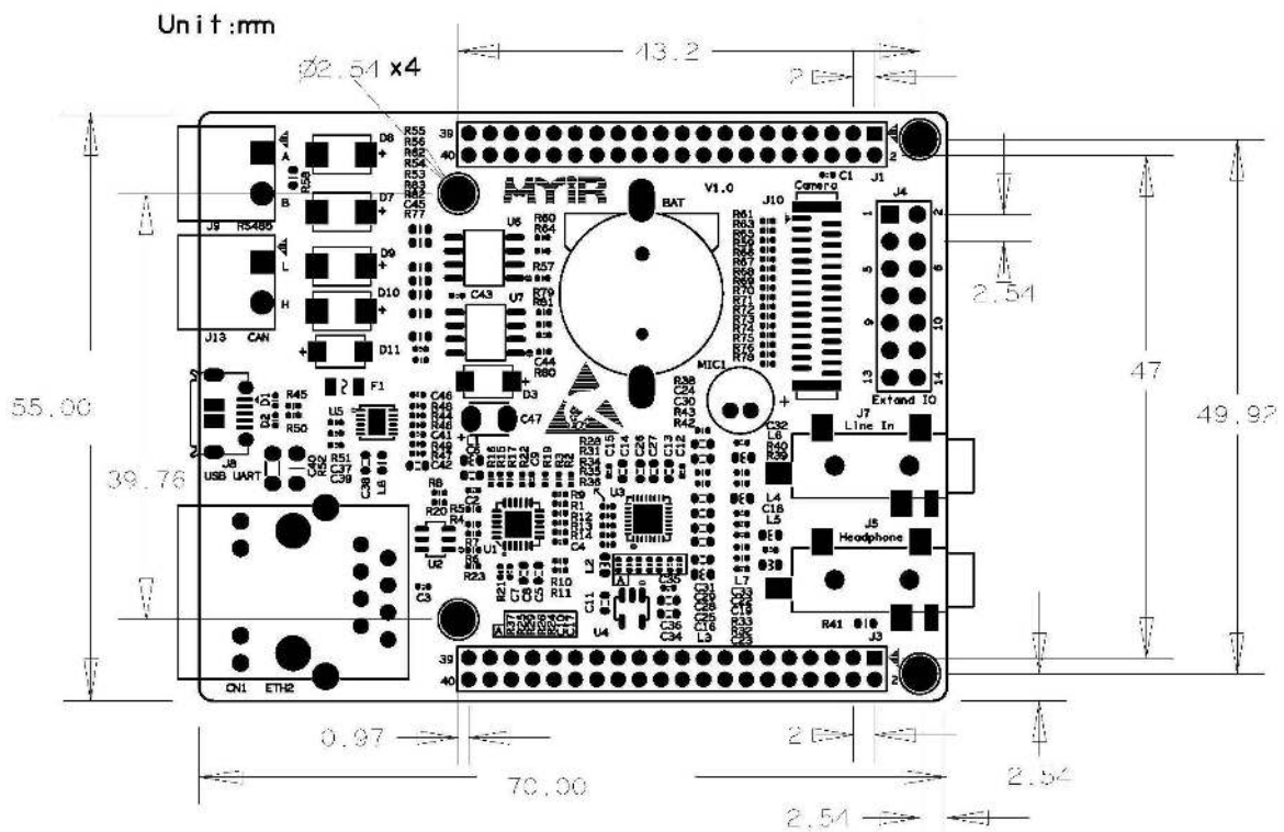
Dimension Chart of MYB-6ULX Expansion Board
