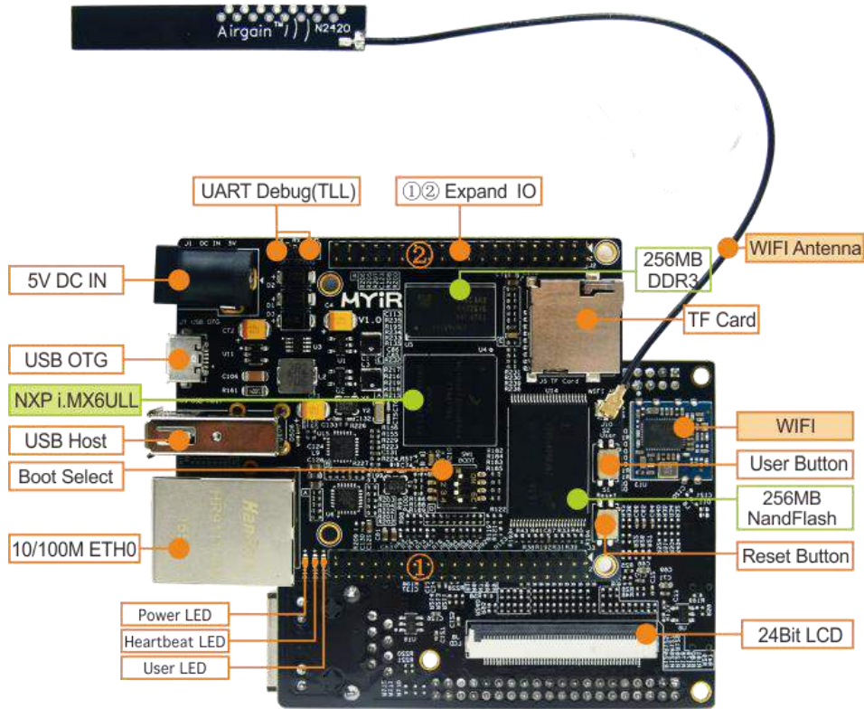
MYS-6ULX-10T
