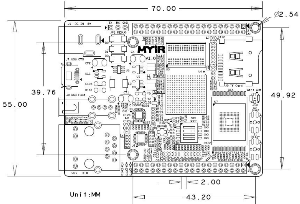
Dimension Chart of MYS-6ULX Single Board Computer
