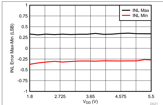
Figure 41. Integral Linearity Error vs Supply Voltage
