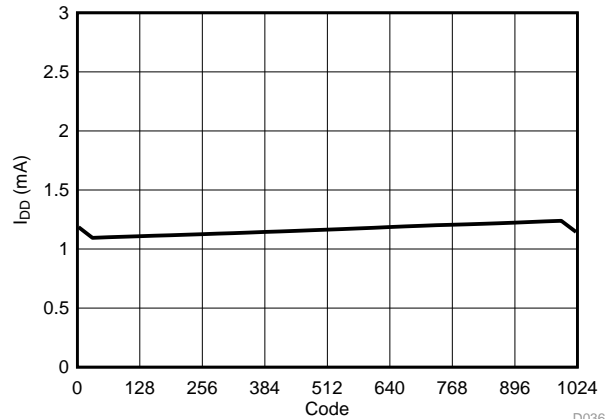
at V_{DD} = 5.5\text{ V} and reference = 5.5 V Figure 25. Supply Current vs Digital Input Code
