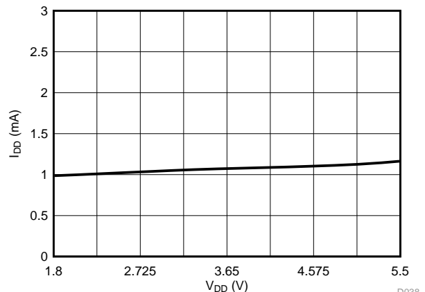
DAC code at mid-scale and reference tied to V_{DD} Figure 27. Supply Current vs Supply Voltage
