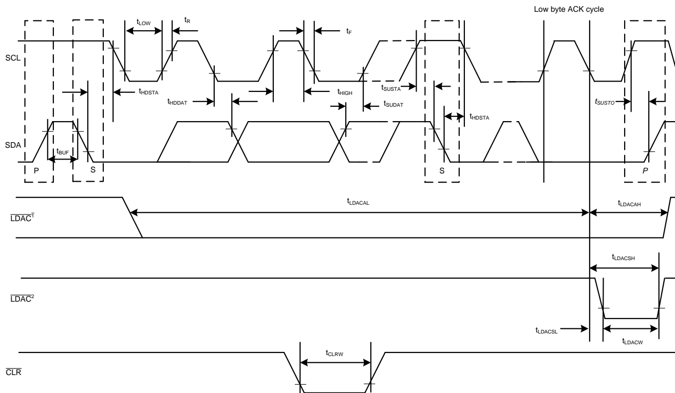
Figure 1. Serial Interface Timing Diagram
