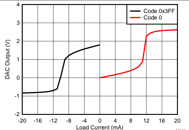
at V_{DD} = 1.8\text{ V} and reference = 1.8 V Figure 29. Source and Sink Capability
