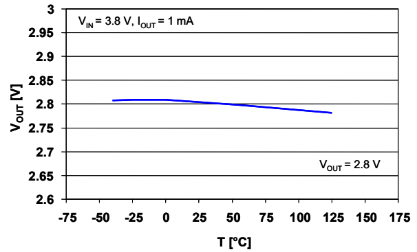
Figure 5. Output voltage vs. temperature ( V_{OUT} = 2.8 \text{ V} )
