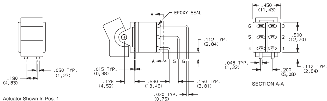
E201J1V5BE2 Vertical Actuation DPDT
