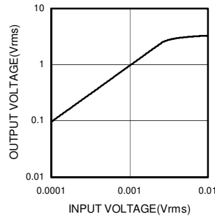
Fig.17 Output Voltage - Input Voltage (PB)
