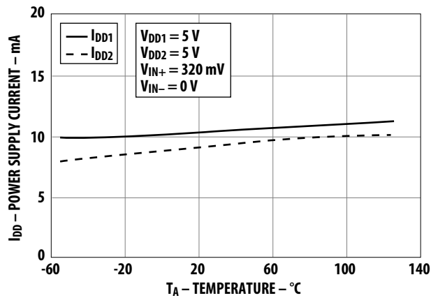
Figure 16 Input and Output Supply Current vs. Temperature
