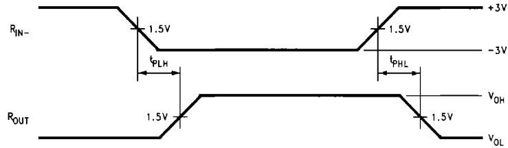
FIGURE 5. Receiver Propagation Delay Waveform
