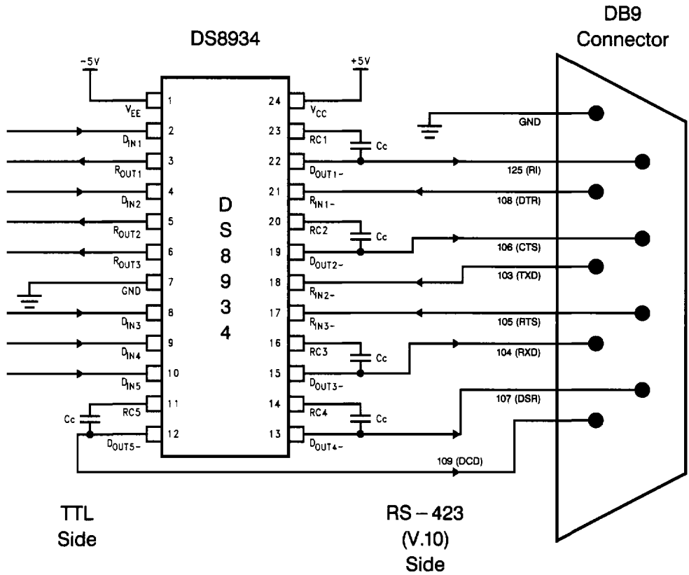
FIGURE 6. Typical V.34 9-Pin DCE Application
