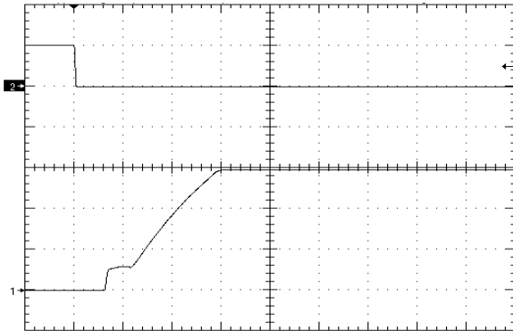
Figure 7. Startup Waveform via Enable Pin, time scale 10mS/div. Vin=Vin_nom, full resistive load (negative enable.) Ch1=5V/div,Ch2=5V/div
