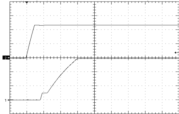
Figure 8. Startup Waveform via Line Voltage, time scale 10mS/div. Vin=Vin_nom, full resistive load + 440uF. Ch1=10V/div,Ch2=20V/div
