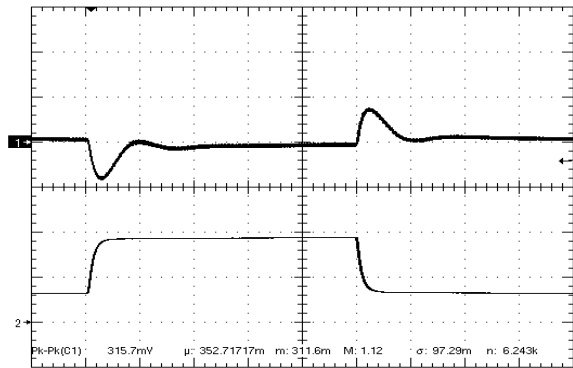
Figure 10. Load Transient Response (200mV/div), di/dt=0.1A/uS, 25% - 75% - 25% of full load +440uF output capacitance, time scale: 200uS/div
