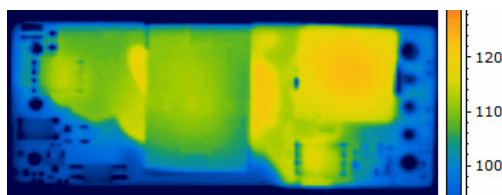
Thermal Image of module @ 48Vin 45C, 200LFM @ Full Load
