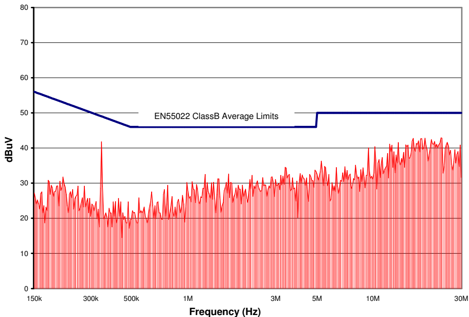
Figure 16. CPE5R48 Conducted Emissions using above specified input filter, Vin = 48V, Full Resistive Load
