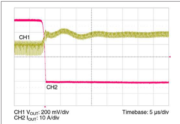
Figure 13 – 50 A – 0 A transient response: C IN = 100 μF, no external C OUT
