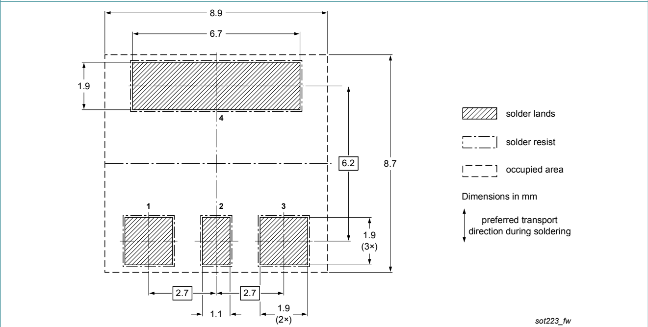
Fig. 10. Wave soldering footprint for SC-73 (SOT223)
