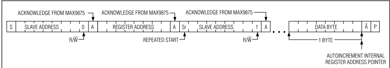
Figure 12. Reading n -Bytes of Indexed Data from the MAX9875
