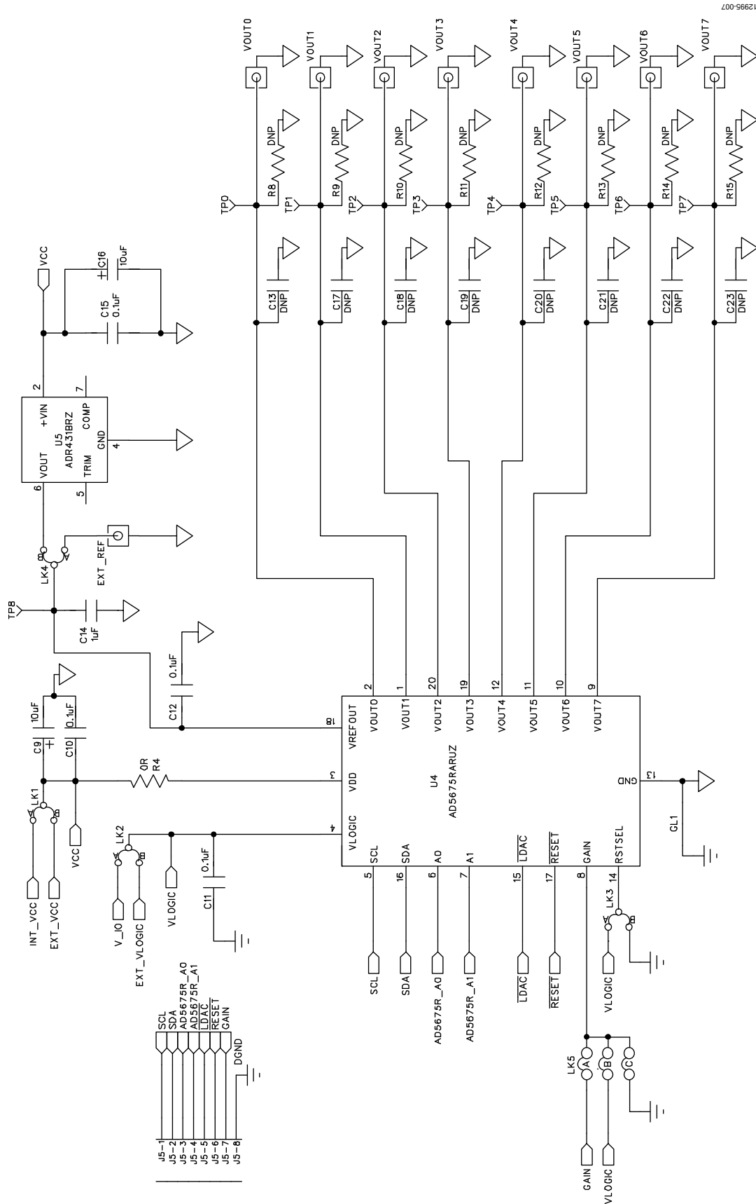
Figure 9. EVAL-AD5675SDZ/EVAL-AD5675RSDZ Schematic, Page 2 of 2
