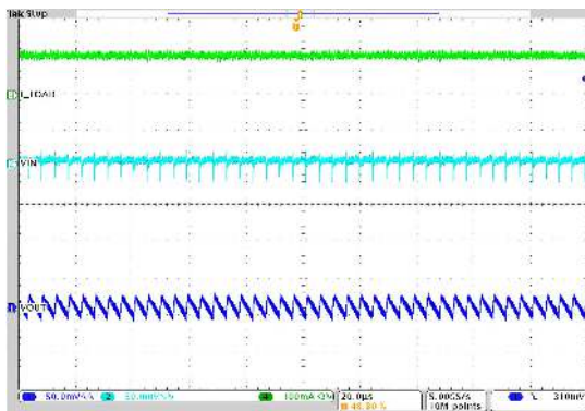
V_{IN} = 12\text{ V} 1-MHz Auto PFM/PWM I_O = 0.1\text{ A} V_{OUT} = 1.2\text{ V} T_A = 25^\circ\text{C}
