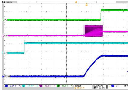
V_{IN} = 12\text{ V} 2.5-MHz PFM/PWM I_O = 1\text{ A} V_{OUT} = 5\text{ V} T_A = 25^\circ\text{C}
