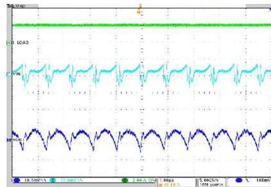
V_{IN} = 12\text{ V} 2.5-MHz Auto PFM/PWM I_O = 2\text{ A} V_{OUT} = 1.2\text{ V} T_A = 25^\circ\text{C}
