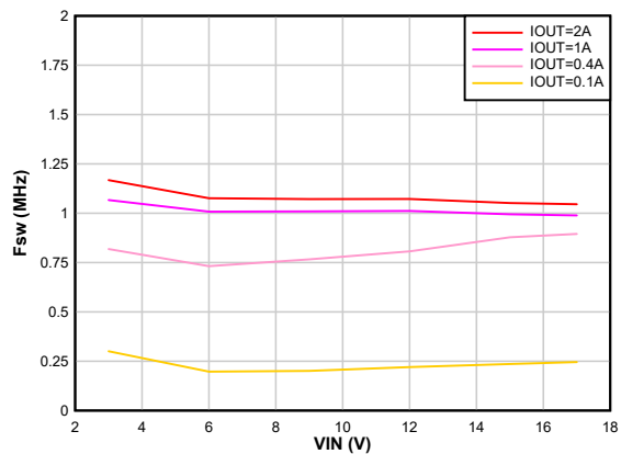
Auto PFM/PWM F_{sw} = 1 MHz
