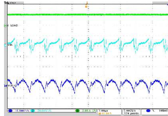
V_{IN} = 12\text{ V} 1-MHz Auto PFM/PWM I_O = 2\text{ A} V_{OUT} = 1.2\text{ V} T_A = 25^\circ\text{C}
