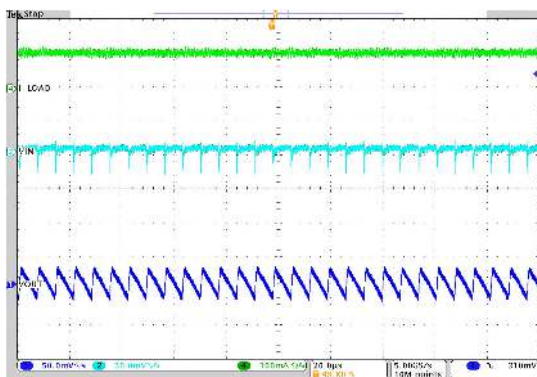
V_{IN} = 12\text{ V} 2.5-MHz Auto PFM/PWM I_O = 0.1\text{ A} V_{OUT} = 1.2\text{ V} T_A = 25^\circ\text{C}
