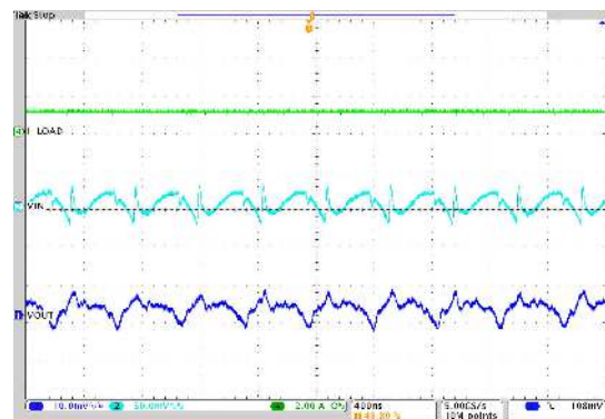
V_{IN} = 12\text{ V} 2.5-MHz Auto PFM/PWM I_O = 1\text{ A} V_{OUT} = 3.3\text{ V} T_A = 25^\circ\text{C}
