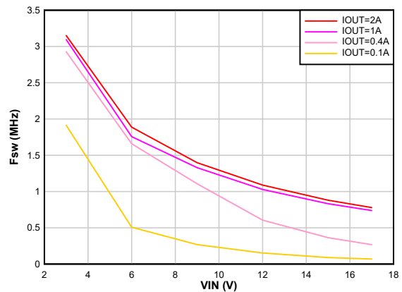
Auto PFM/PWM F_{sw} = 2.5 MHz
