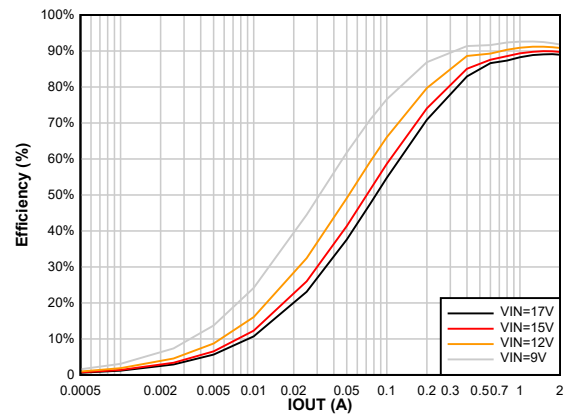
FPWM F_{sw} = 2.5 MHz
