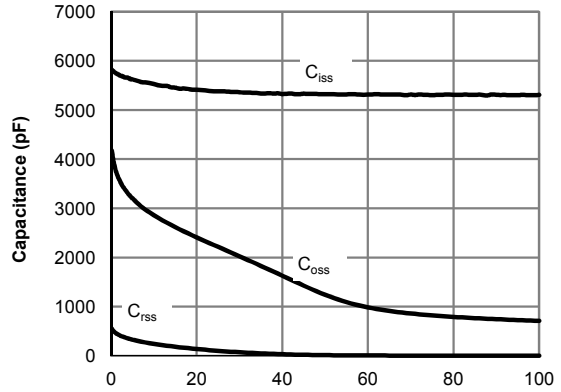
Figure 8: Capacitance Characteristics
