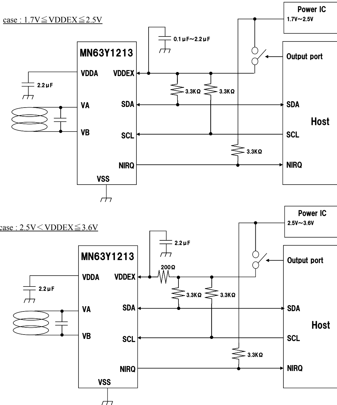
Figure 2-3 Connection Example
