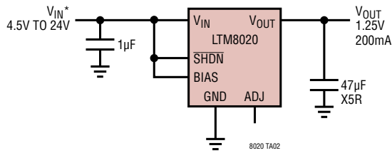
1.25V Step-Down Converter
