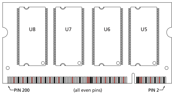
Figure 2: Module Layout
