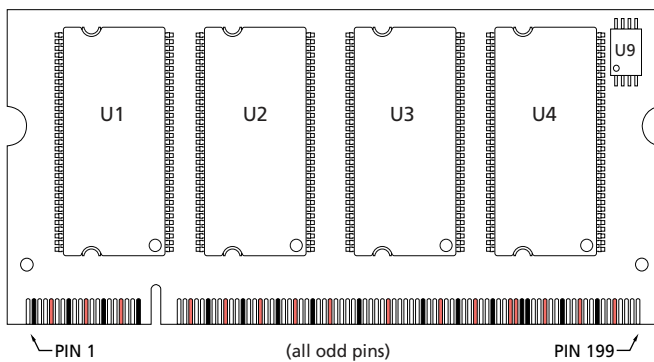
Figure 2: Module Layout
