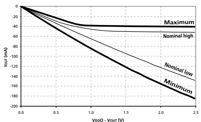
Figure 9: Pull-Up Characteristics
