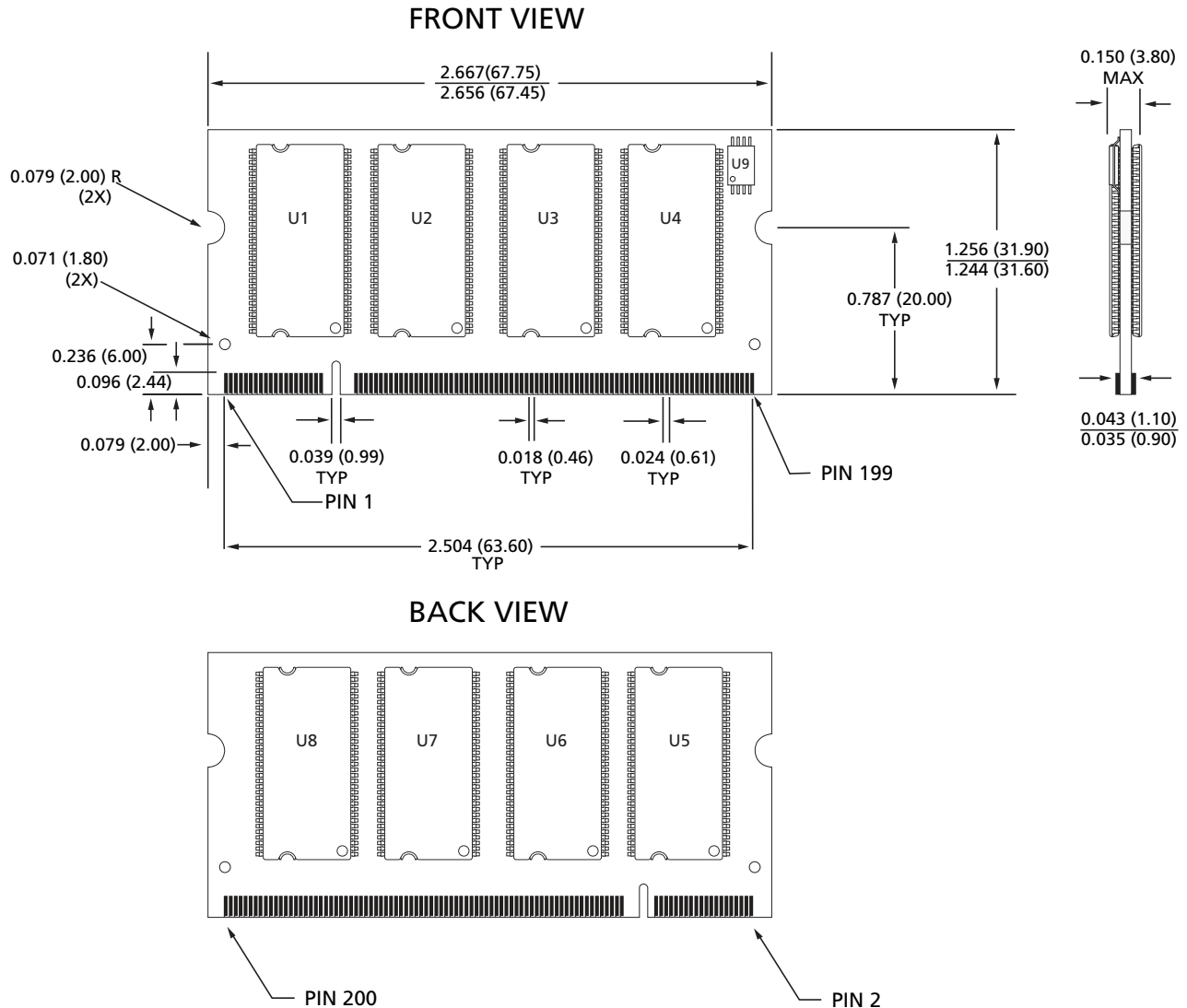
Figure 15: 200-Pin DDR SODIMM Dimensions
