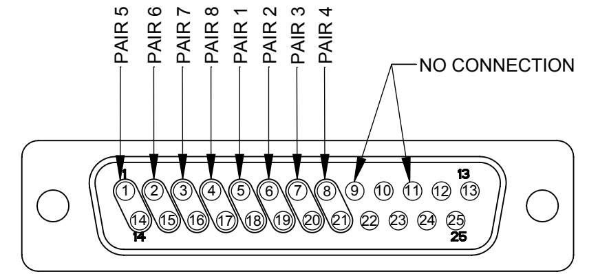
DB25 PIN-OUT VIEW
