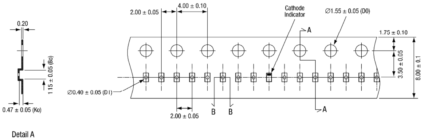
Figure 9. SOD-882 Package Dimension Drawing
