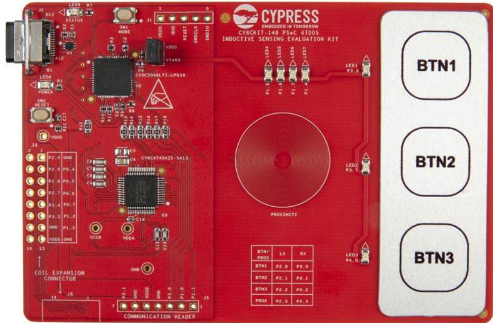
Figure 1-1. CY8CKIT-148 PSoC 4700S Inductive Sensing Evaluation Kit
