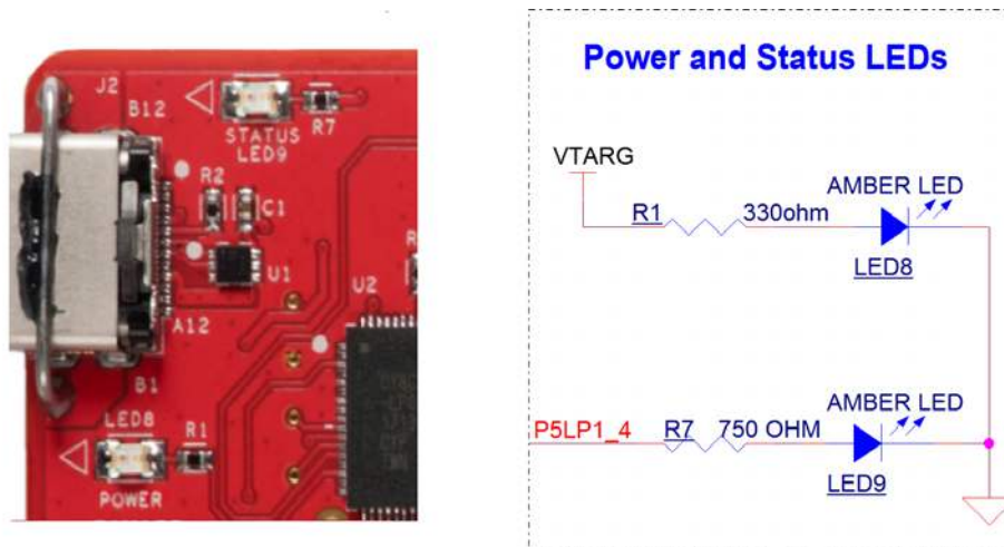
Figure A-16. Power and Status LEDs
