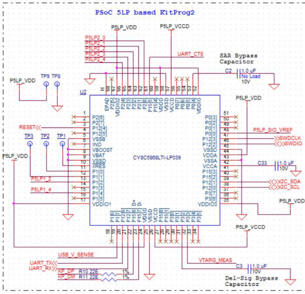
Figure A-3. Schematic of PSoC 5LP (KitProg2)
