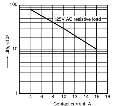
4. Life curve Operation frequency: 20 times/min. (ON/OFF = 1.5s:1.5s) Ambient temperature: Room temperature
