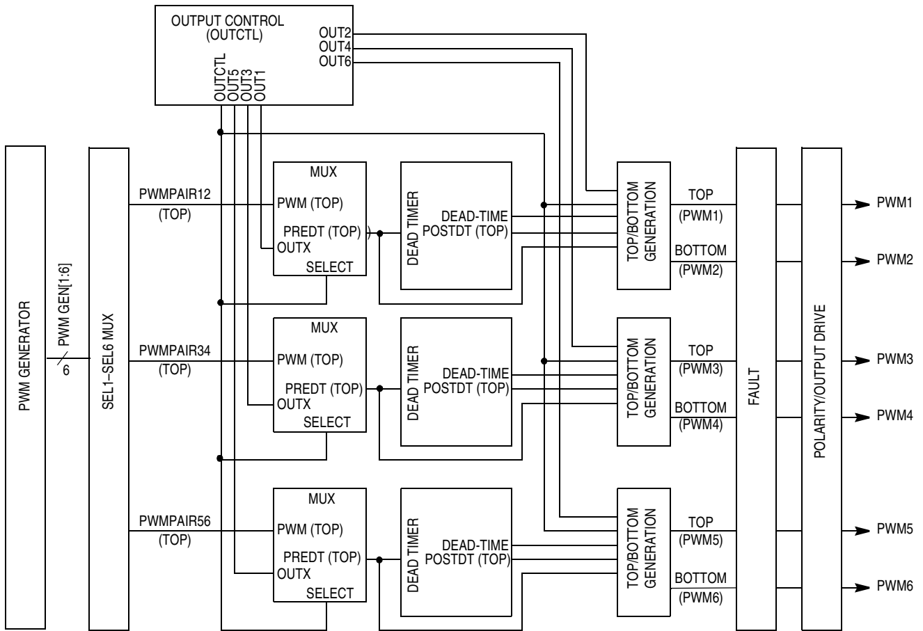
Figure 9-13. Dead-Time Generators
