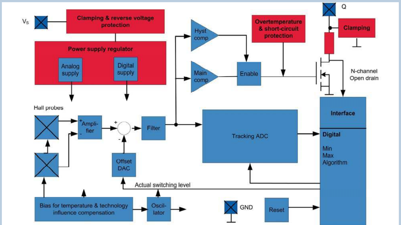
Block Diagram
