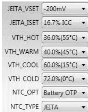
Figure 17: NTC Functions Settings
