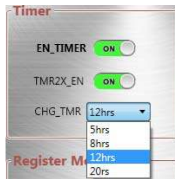
Figure 20: Charge Timer Setting
