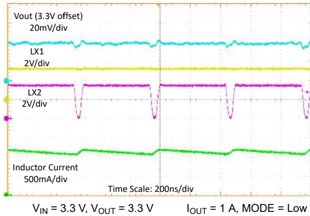
Figure 9-8. Switching Waveforms with 1-A Load
