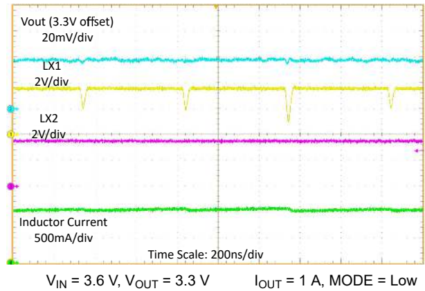
Figure 9-9. Switching Waveforms with 1-A Load
