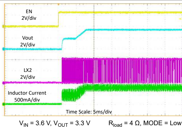
Figure 9-12. Start-Up by EN
