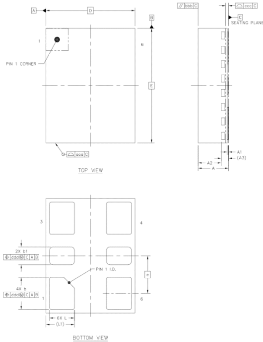
Figure 5.2. AS5002 (2.5 x 3.2 mm) Outline Diagram
