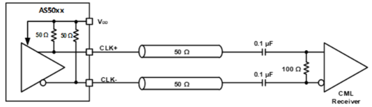
AC-Coupled CML
