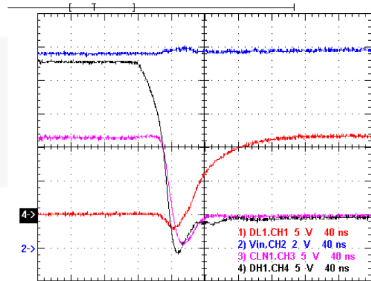
Figure 16. Dead Time with Heavy Load (Fall Edge)
