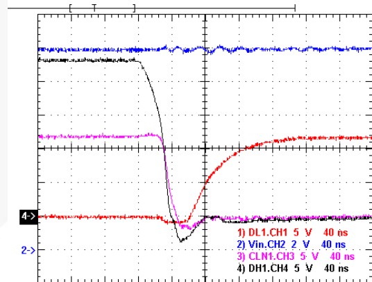
Figure 14. Dead Time with Light Load (Fall Edge)
