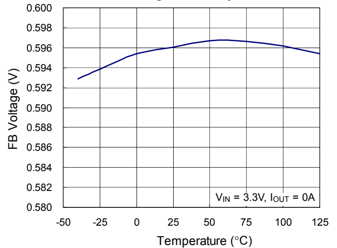
FB Voltage vs. Temperature
