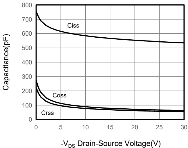
Figure 5. Capacitance
