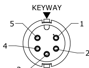
FACE VIEW ASSY: 6280-5SG-5XX
