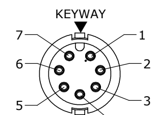
FACE VIEW ASSY: 6280-7SG-5XX
