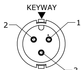
FACE VIEW ASSY: 6280-3SG-5XX
