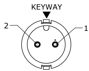
FACE VIEW ASSY: 6280-2SG-5XX
