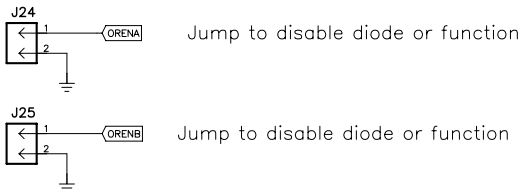
Figure 6. TPS2456 Schematic
