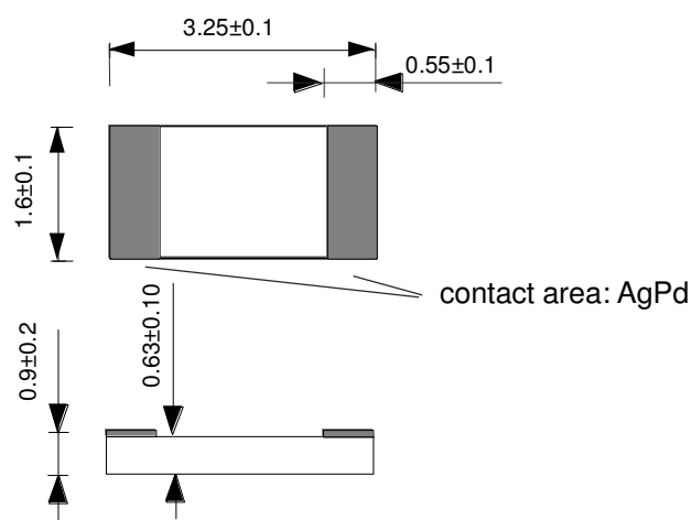
Figure 1: Mechanical dimensions of Platinum Temperature Sensor
