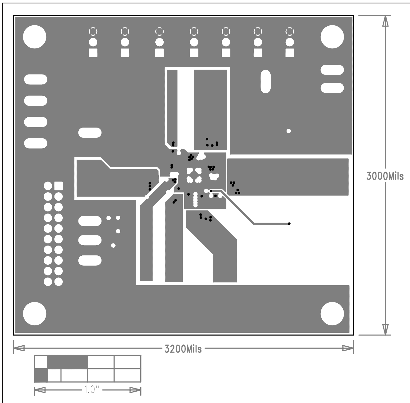
Figure 8. MAX8660 EV Kit PCB Layout—Power Layer 3
