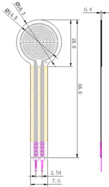
RP-C18.3-LT Dimension Diagram
