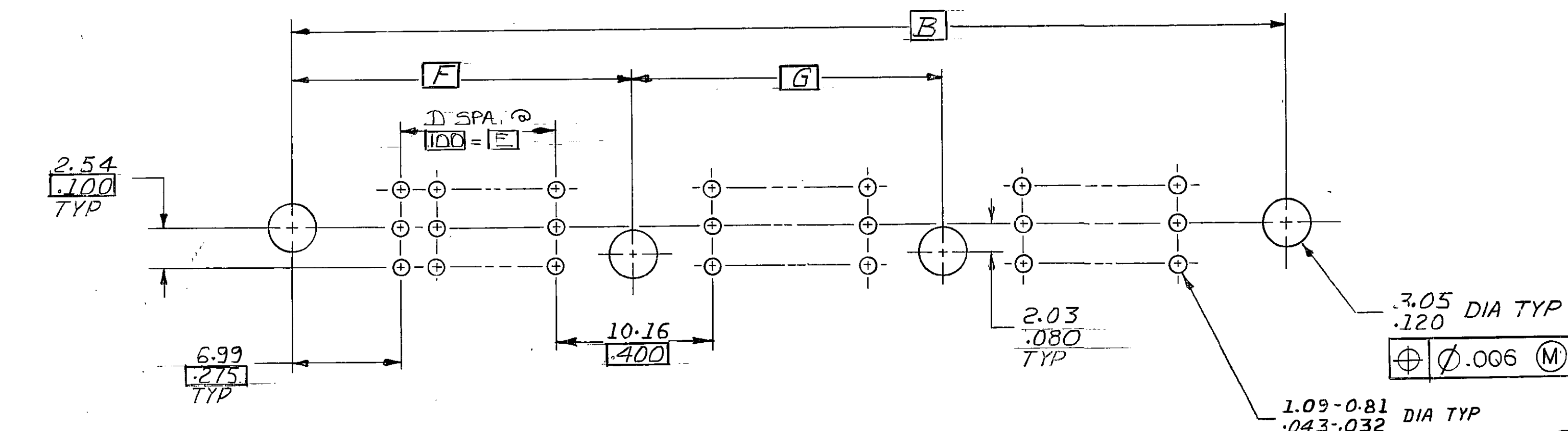
RECOMMENDED P.C. BOARD HOLE LAYOUT
