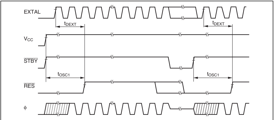
Figure 20.5 Oscillation Stabilization Timing
