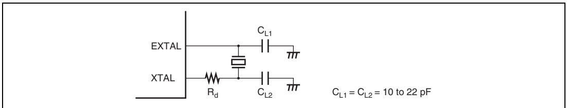
Figure 17.2 Typical Connection to Crystal Resonator
