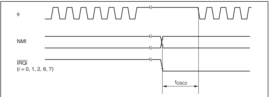
Figure 20.6 Oscillation Stabilization Timing (Leaving Software Standby Mode)
