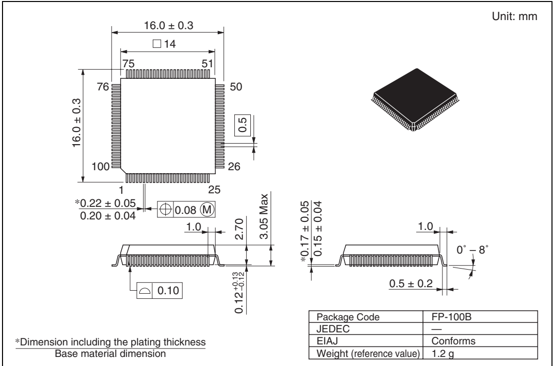
Figure C.1 Package Dimensions (FP-100B)
