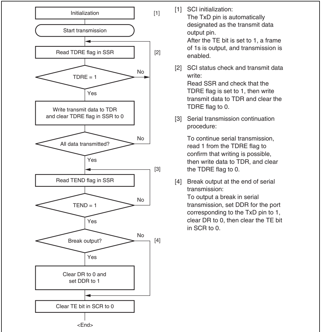
Figure 12.7 Sample Serial Transmission Flowchart
