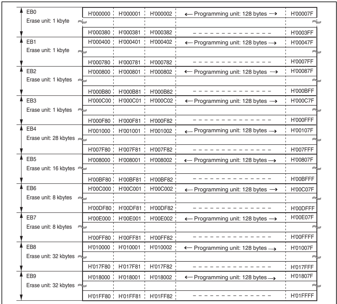
Figure 16.5 Flash Memory Block Configuration
