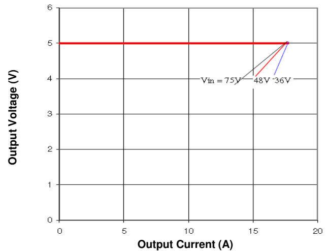
Figure 10. Output Characteristics
