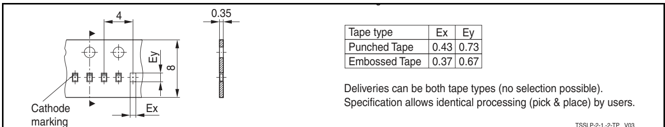
Figure 6-3 PG-TSSLP-2-1: Packing
