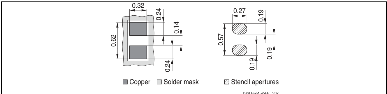
Figure 6-2 PG-TSSLP-2-1: Footprint
