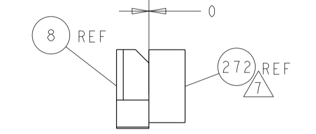
TERMINAL SUPPORT LOCATION FOR TERMINAL PN 1949499-1
