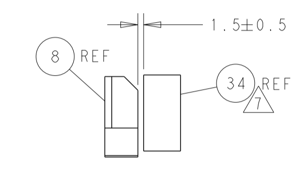
TERMINAL SUPPORT LOCATION FOR TERMINAL PN 1949498-1
