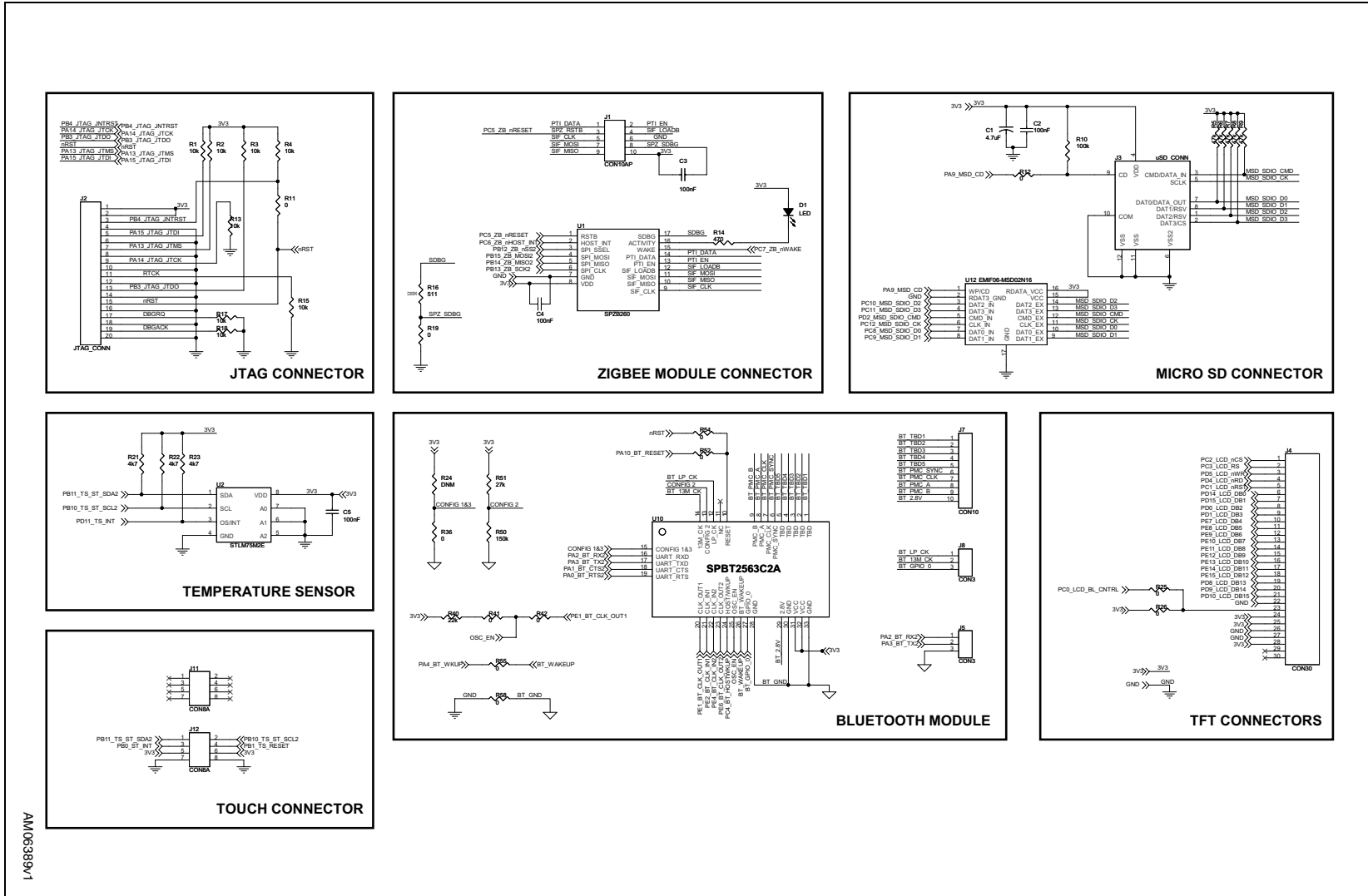
Figure 2. Connector circuit schematics
