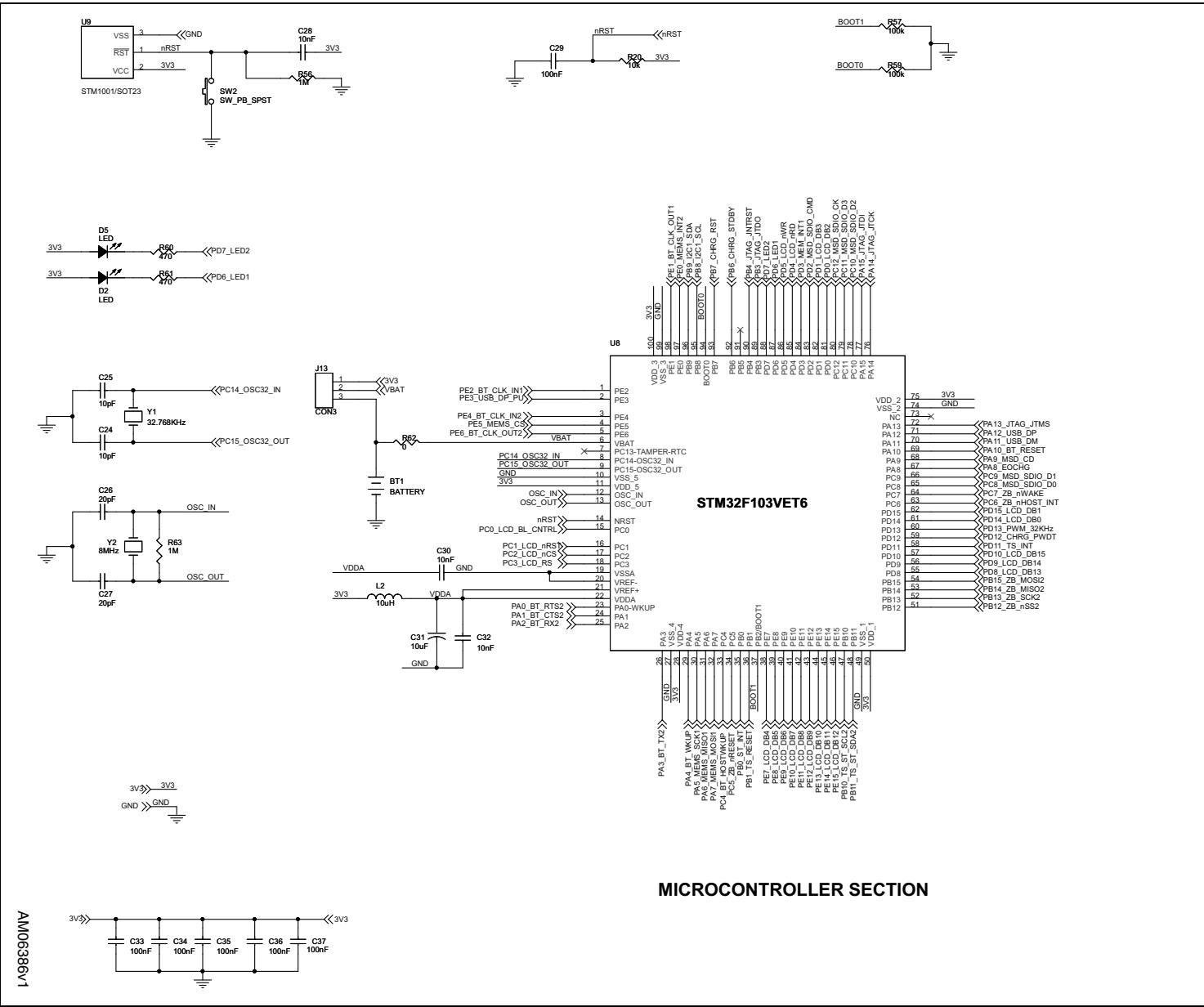
Figure 1. Microcontroller circuit schematic
