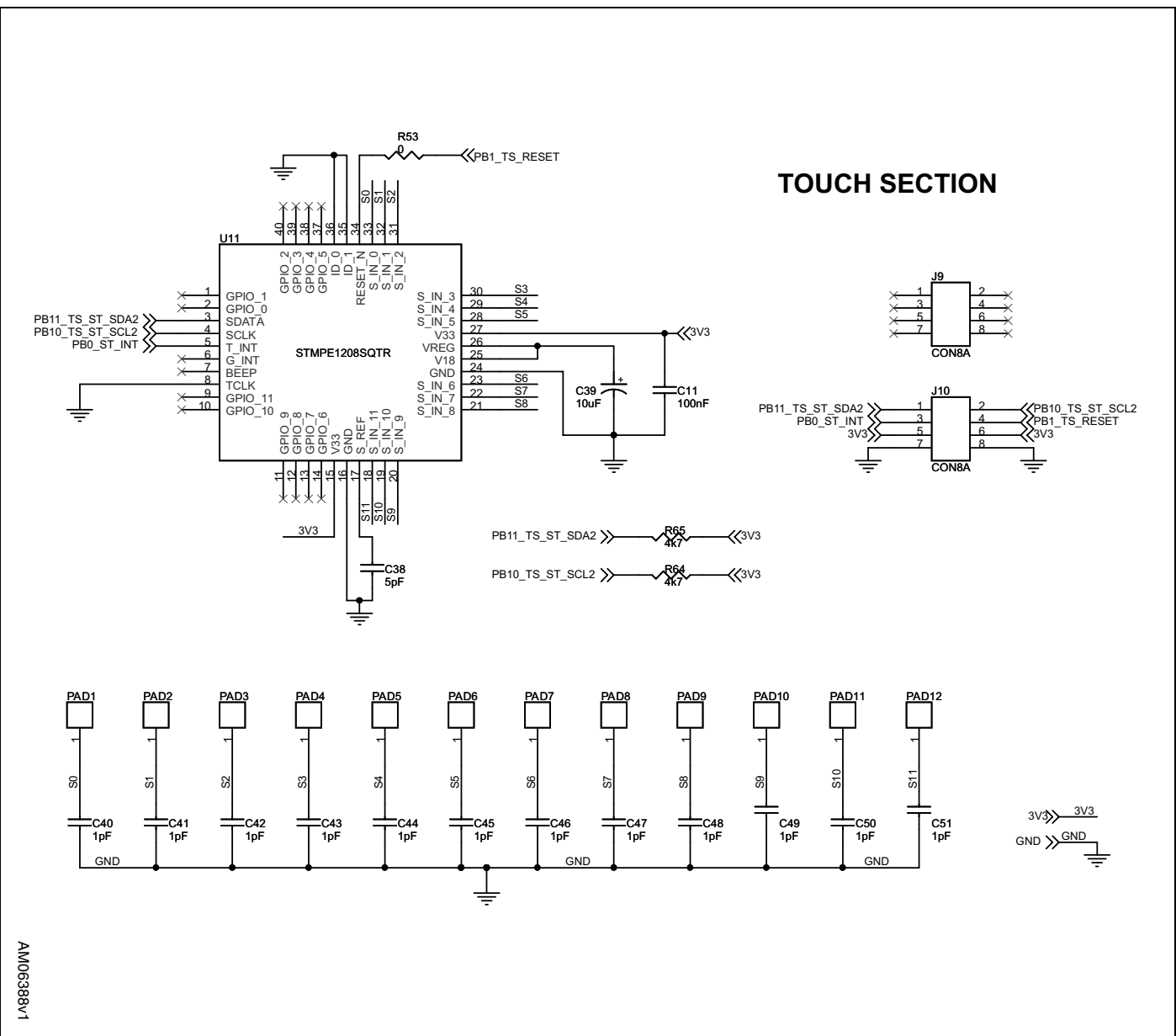
Figure 4. Touch section schematic
