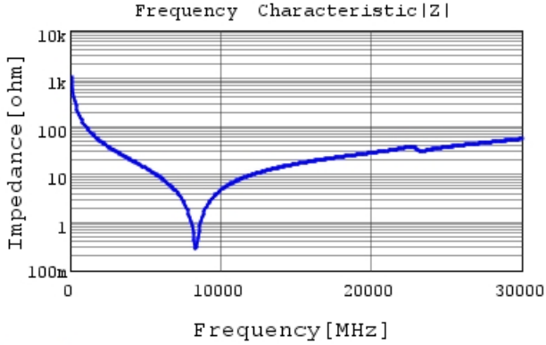
GJM0335C1E1R5CB01 |Z| DC0V, 25degC
