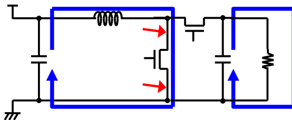
Figure 1. MOSFET-ON
