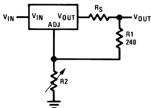
Figure 16. Regulator With Line Resistance in Output Lead
