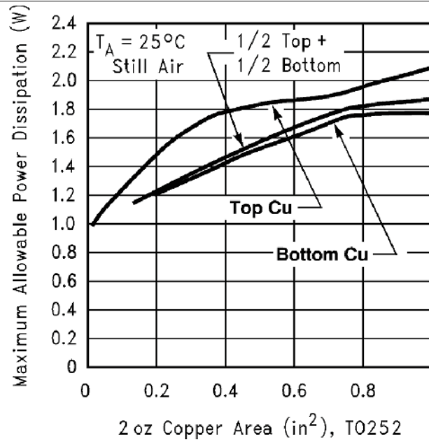
Figure 45. Maximum Allowable Power Dissipation vs 2-oz. Copper Area for TO-252
