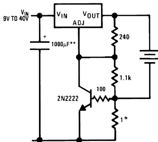
Figure 34. Current-Limited 6-V Charger
