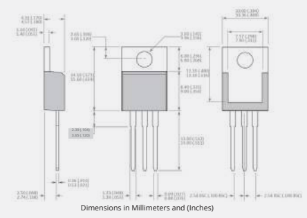
TO-220 3-Lead
