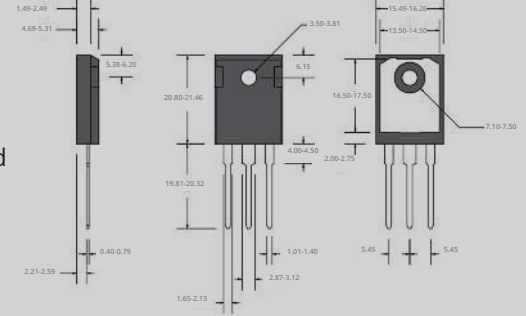
TO-247-3-Lead
