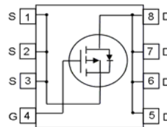
PG-DSO-8
